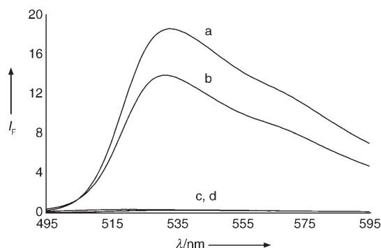
Figure 3. Fluorescence intensity ( I_F ) of 1 K \gamma -PNAs with thiazole orange attached to the side chains: a) PNA 13 combined with the complementary DNA; b) PNA 12 combined with the complementary DNA; c) PNA 13 by itself; and d) PNA 12 by itself.
